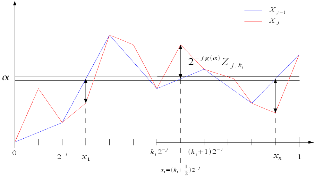
Figure 4: The processes X_{j-1} and X_j .
