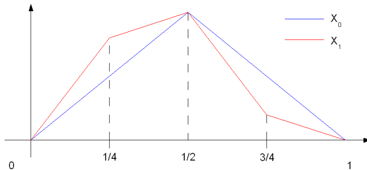
Figure 1: Processes X_0 and X_1 .
