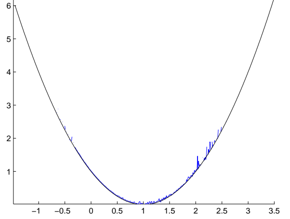
Figure 5: Estimation of the self-regulating function for an srmdp sampled on 65536 points with two values for \varepsilon .
