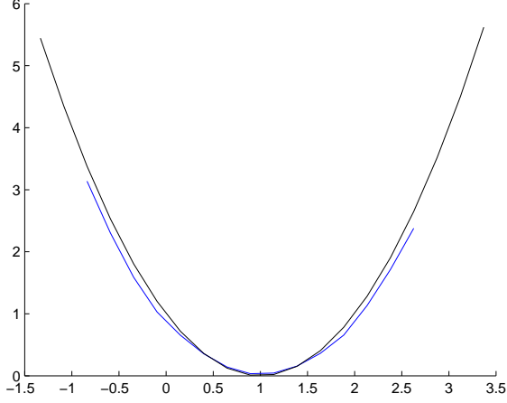
Figure 5: Estimation of the self-regulating function for an srmdp sampled on 65536 points with two values for \varepsilon .
