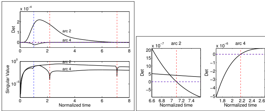
Fig. 5 Fluid case, step 4: second order conditions. Second order necessary condition check on solution 1/12 with \lambda = 2.0 from Table 3. The rank condition from the algorithm presented in subsection 4.3 from [11] is evaluated along the two singular arcs. See [6] for details on the concept of conjugate times. On the left subplot, for each singular arc, the curve is reparameterized so that the final time corresponds to the abscissa 1 (vertical blue dashed line); the determinant associated with the rank condition is plotted (top subgraph), so there is a conjugate time whenever it vanishes (vertical red dashed lines). One observes that conjugate times on each arc are located after the (normalized to 1) final time, satisfying necessary condition of local optimality of the trajectory. At the bottom, the smallest singular value of the matrix whose rank we test is plotted, extracting only the relevant information to detect the rank drops. On the right subplot is presented a zoom of top-left subgraph near the two conjugate times.
