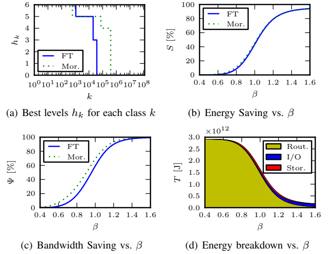
Fig. 1. Best levels for each class k (a) and impact of the variation of \beta (b-d).
