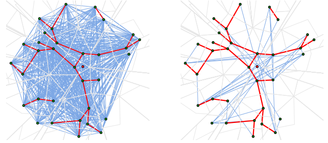
Figure 4. Left: In the case of unknown doublets and triplets, naïvely, all possible pairs of points have to be considered. Right: Our geometric constraints are able to remove most of the false connections.
