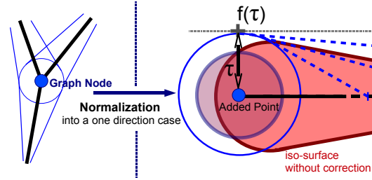
Figure 14: Correction of the scalar field around a node of maximal radius in the skeleton graph. A "normalized" version of the node is used to compute the lacking field value.
