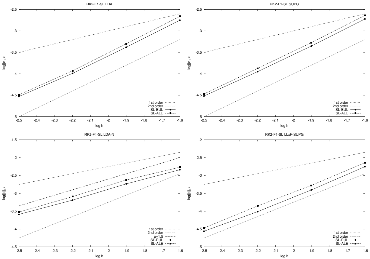
Figure 14: Advection of a vortex. Order of Convergence fig:VortAdv
