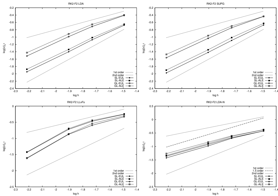
Figure 3: Linear Advection. Order of Convergence fig:Linear-Advection
