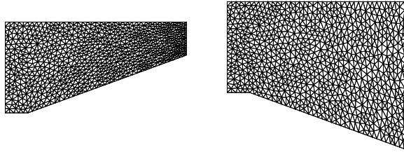
Figure 20: Topology for the grid. Left: compression. Right: expansion. fig:Mapping_for_wind_tunn
