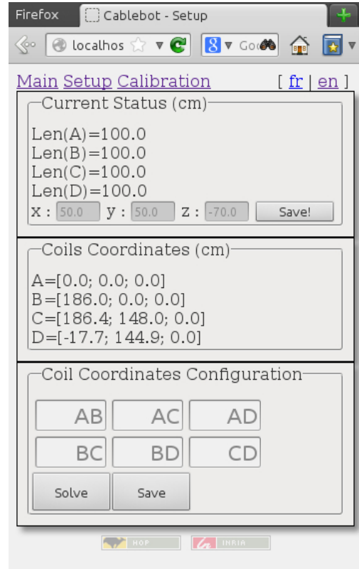
Figure 3: The configuration interface
