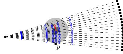
Figure 8: Shewchuk's edge protection applied to a problematic case. The PLC contains the black disks and dashed segments, the small circles show the Steiner points constructed to embed the segments. The red Steiner points are incident to two edges that are too short, the gray disks show the edge length and four times this distance disproving his Theorem 2.
