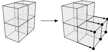
Fig. 4. The extrusion of the lower row of two faces.
