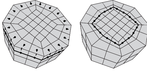
Fig. 6. Left: A dual cycle on a surface mesh (marked with thick solid lines). The dashed lines are the neighboring dual edges to one of the cycles sides (with respect to its orientation). In this example, the corresponding primal edges all have a sharp dihedral angle and thus the presented dual cycle's weight is high. Right: An illustration of a flat cycle on a planar surface region. The elimination of these cycles should be avoided.
