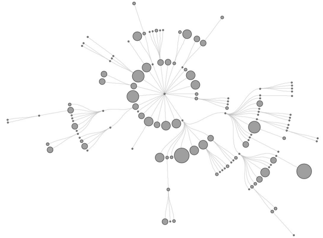
Figure 1: Radial-Tree Layout
