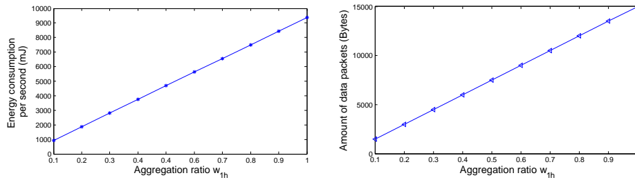
(a) The energy consumption with different aggregation ratio w_{1h} (b) The capacity with different aggregation ratio w_{1h}
