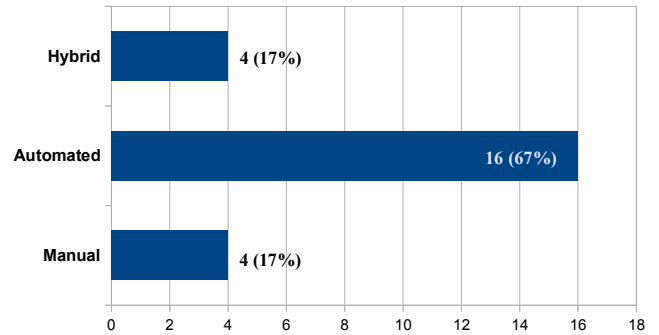
Fig. 2 Strategy human intervention degree analysis
