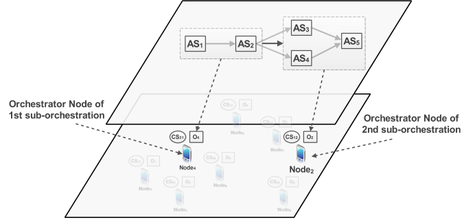
Fig. 8: The third DoF: sub-orchestrator selection
