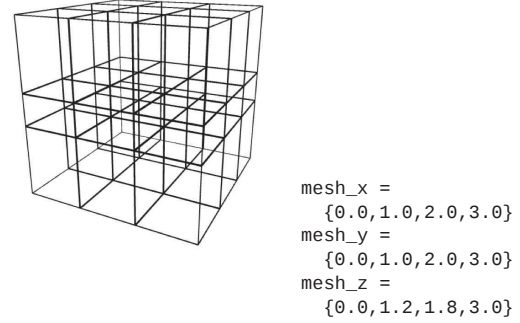
Figure 2: Example of a 4x4x4 rectilinear grid described by three arrays of coordinates. In this example there is one scalar value (such as temperature or wind velocity ) at each node.
