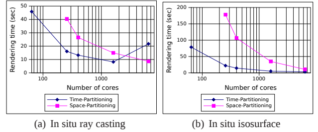
Figure 4: Rendering time using ray-casting and isosurfaces, with time-partitioning and space-partitioning with CM1. Note that the number of cores represents the total number; using a space-partitioning approach, 1/16 of this total number is effectively used for in situ visualization.
