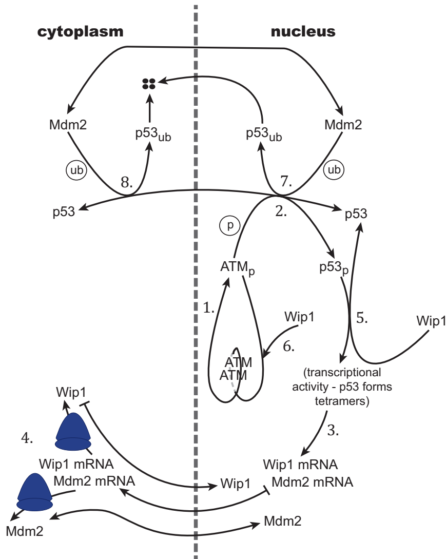
Figure 3: p53 dynamics under stress conditions: 1. ATM autophosphorylation (a consequence of the exposure to stress conditions, e.g., \gamma -radiation) results in ATM dimer dissociation into active monomers ATM_p , which, 2., can phosphorylate p53 ( ATM_p and p53_p do not leave the nucleus). 3. Phosphorylated p53 forms tetramers which bind DNA and act transcriptionally for Mdm2 and Wip1. 4. The mRNAs of the proteins leave the nucleus, bind ribosomes and they are translated into proteins; Wip1 moves into the nucleus only while Mdm2 acts in both compartments. 5. Wip1 dephosphorylates p53_p , making it visible for Mdm2. 6. Wip1 also dephosphorylates ATM_p which dimerises with another dephosphorylated ATM molecule. Dephosphorylated p53 can freely migrate between the compartments, where, 7. and 8., it can be ubiquitinated by Mdm2 and subsequently degraded. Arrows in this sketch either indicate directions of molecule migrations, uni- or bidirectional, T-shaped lines meaning impossible nucleocytoplasmic transport in the T-end direction, or schematically show reactions in the signalling pathways.
