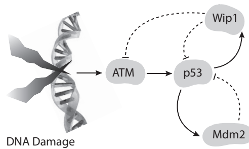
Figure 1: The studied p53 dynamics: in response to DNA damage, ATM is activated and phosphorylates p53, which results in inhibition of the p53–Mdm2 compound formation; p53 accumulates in the nucleus and acts as a transcription factor for Mdm2 and Wip1; Wip1 dephosphorylates ATM and p53 keeping them inactive and enabling Mdm2 to bind p53 again, Mdm2 initiates ubiquitination of p53, its nuclear export and degradation.
