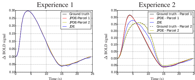
Fig. 1. Ground truth and estimated HRFs using JDE and JPDE.
