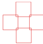
(b) ROCircleLayout
