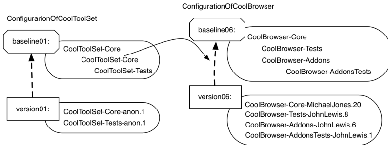
Figure 9.8: Dependencies between configurations.
