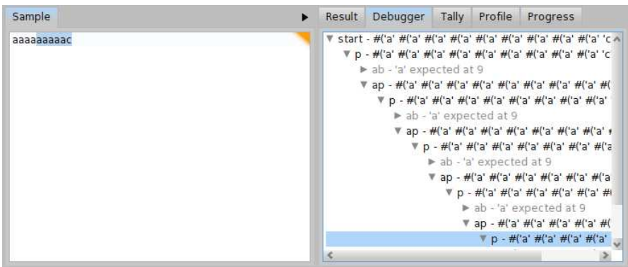
Figure 18.29: Debugging output of BacktrackingParser for input c .
