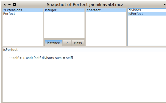
Figure 7.14: The snapshot browser reveals that the Perfect package extends the class Integer with 2 methods.
