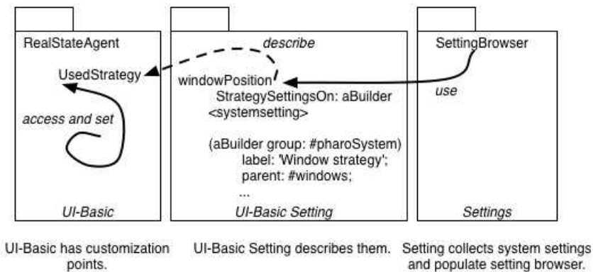
Figure 5.1: A package defines customization points. Such customization points are described with Settings instances. The Settings Browser collects the description and presents them to the user.
