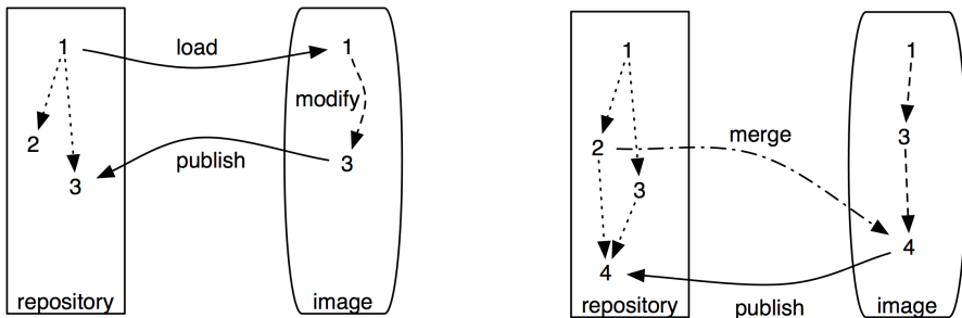
Figure 7.10: Branching (left) and merging (right).
