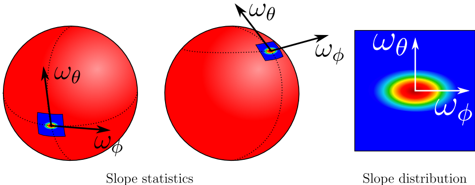
Figure 4: We use a noise primitive that produces Gaussian slope statistics (\sigma_\theta, \sigma_\phi) at any local frame (\omega_\theta, \omega_\phi) on the sphere. The noise statistics are constant in world space and are not affected by the spherical parameterization.
