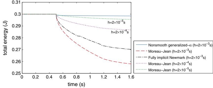
Figure 10. Numerical results for the total energy of the bouncing elastic bar.
