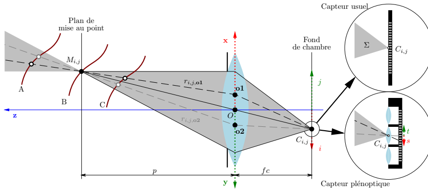
Figure 3.4: Differences between standard and plenoptic cameras: from above (axes \mathbf{x}, j, s ) or the side (axes \mathbf{y}, j, t ) the rays converging as a single point at the back wall of the darkroom are summed in the first and differentiated by refraction and sampling in the second
