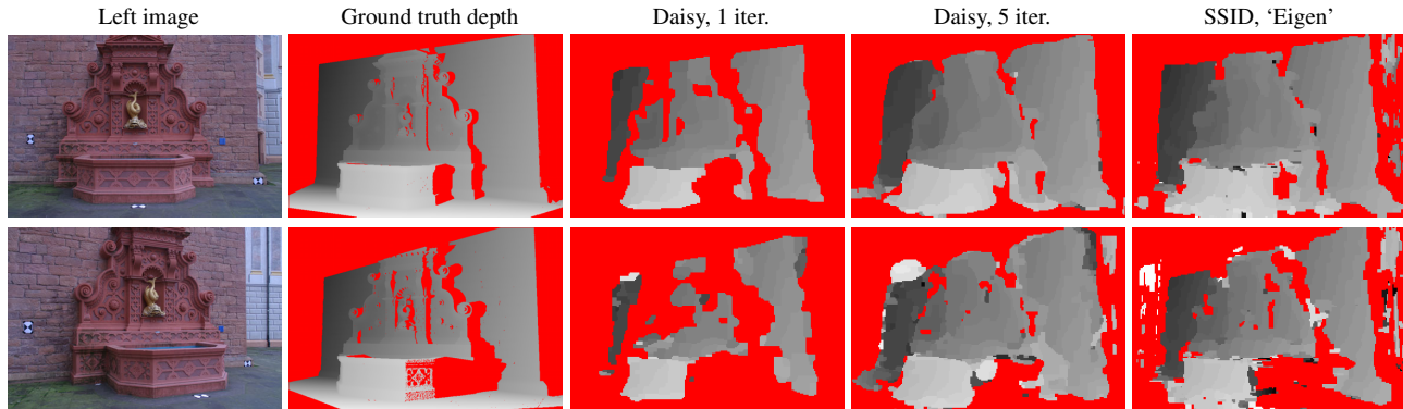
Figure 10. First column: The images on the left (Images 5 and 7 of [31]) are matched against Image 3 of [31], shown is Fig. 2, which serves as the the ‘Right image’), for an increasing baseline. Second column: ground truth depth maps of [31]. Third and fourth columns: first and fifth iteration of the Daisy stereo algorithm. Fifth column: single shot depth estimation with SSID and ‘Eigen’ embeddings. The occlusion estimates for the first Daisy iteration may seem aggressive, but allow the algorithm to converge. Higher occlusion costs induce errors in the initial estimate and degrade the final accuracy.
