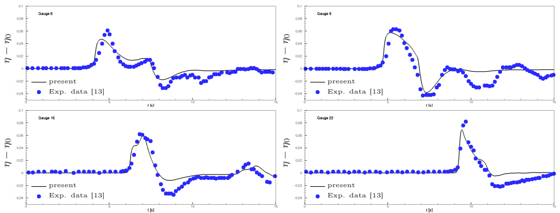
Figure 20: Run up on a conical island [13] : gauge data (left)
