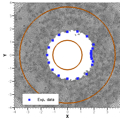
Figure 21: Run up on a conical island [13] : maximum run up plot
