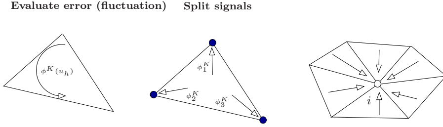
Figure 2: Residual Distribution/Fluctuation splitting methodology
