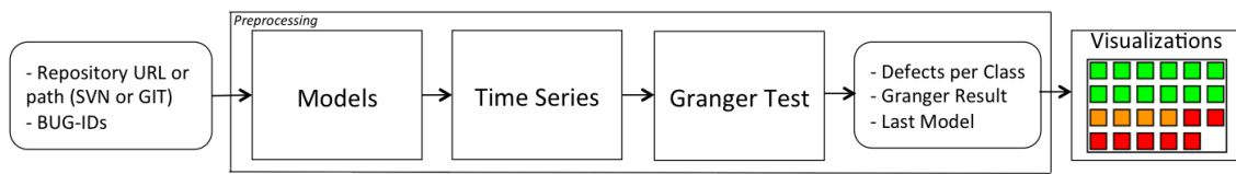
Figure 1. BugMaps-Granger's architecture
