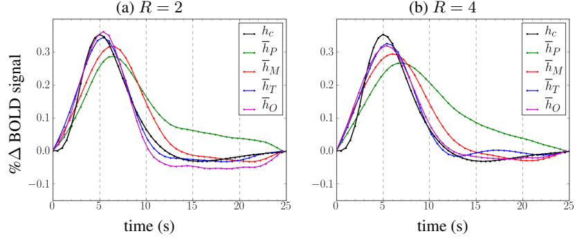
Figure 12: Group-average HRF estimates for acceleration factors R = 2 (a) and R = 4 (b). \bar{h}_P, \bar{h}_M, \bar{h}_T, \bar{h}_O stand for HRF means in parietal, motor, temporal and occipital regions, respectively. h_c stands for the canonical HRF.
