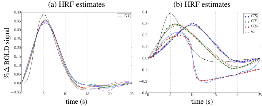
Figure 5: JDE-based HRF estimates for each subject along with the ground truth (denoted GT). (a): In the first simulation scenario, all subjects elicit BOLD responses according to the canonical HRF shape h_c shown in black line . (b): In the second simulation scenario, subject-varying HRFs that deviate from h_c have been used as illustrated by the color coding: 4/2/2 subjects were associated with the ground truth HRFs in blue , green and red shapes, respectively.
