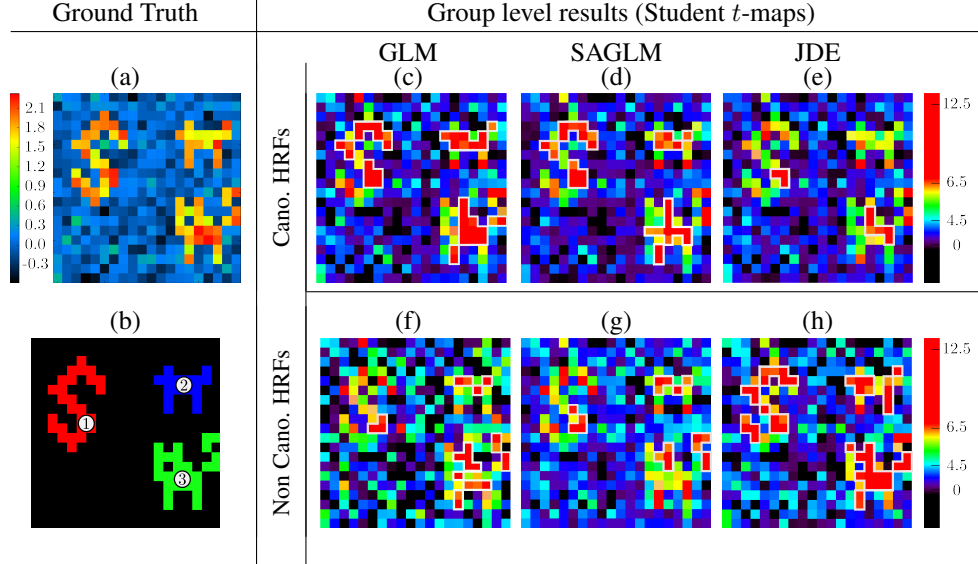
Figure 4: (a): Simulated averaged activity over subjects (true mean NRLs). (b): Spatial configuration of true activation clusters: clust. #1: 26 activated voxels; clust. #2: 16 activated voxels and clust. #3: 28 activated voxels. (c)-(e): Group-level Student t -maps related to the first scenario (simulated canonical HRFs) and obtained for the three intra-subject inference methods (GLM, SAGLM and JDE from left to right). (f)-(h): Group-level Student t -maps related to the second scenario (subject-varying non-canonical HRFs) and obtained for the same methods as above.
