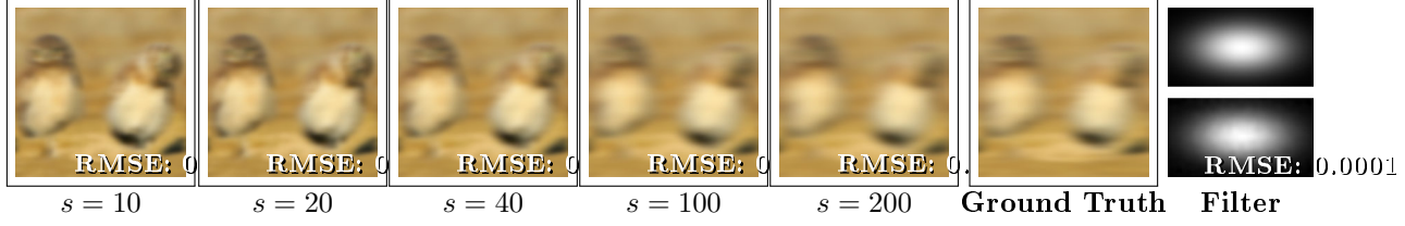
Figure 4: We demonstrate the convergence of IFD filtered images with an increasing number of terms s . Ground truth is computed numerically with a FFT. Our multi-frequency IFD MoG approximation ( bottom-right ) of an anisotropic kernel ( top-right ) obtained with the SpARSA algorithm, and the reconstructed kernel and error using 200 coefficients.
