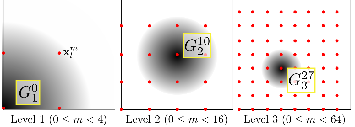
Figure 2: Displacements \mathbf{x}_l^m for MoG kernels G_l^m used in our 2D image IFD, for frequency levels l = \{1, 2, 3\} .
