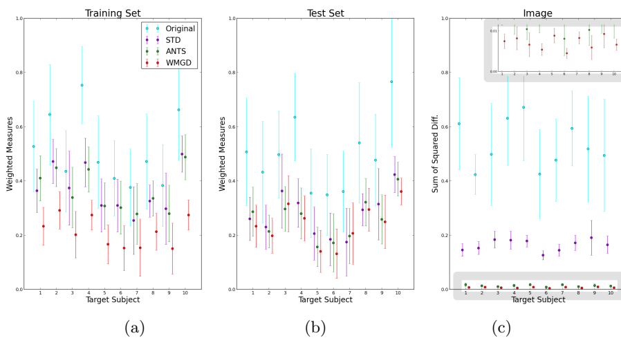
Fig. 3. Registration of the dataset to each subject. STD, ANTS, and WMGD show the average accuracy of the registration to each subject for the corresponding method. Original corresponds to the original distances between the dataset and the chosen target subject. Values were scaled using min-max normalization.
