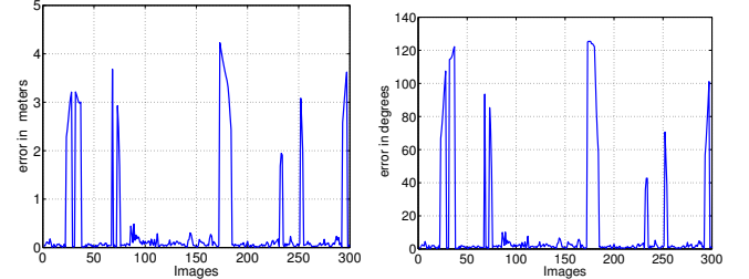
Fig. 8. Error on the estimated pose parameters using method L for the image sequence 1 versus image number: left) \|t_e\| , right) \theta_e .
