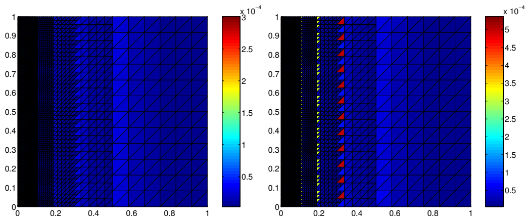
Figure 37: Distribution of the total error (left) and its estimate (right) on the fifth mesh
