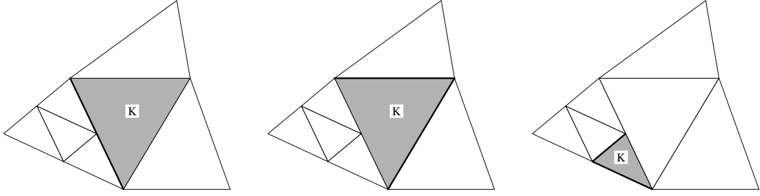
Figure 2: An example of the set of faces (bold lines) \mathcal{E}_K^{\text{HG}} of an element with a hanging node (left), the set of faces \mathcal{E}_K^{\text{HG},\text{N}} of an element with a hanging node (center) and the set of faces \mathcal{E}_K^{\text{HG},\text{N}} of an element whose vertex gives rise to a hanging node of the neighboring element (right).
