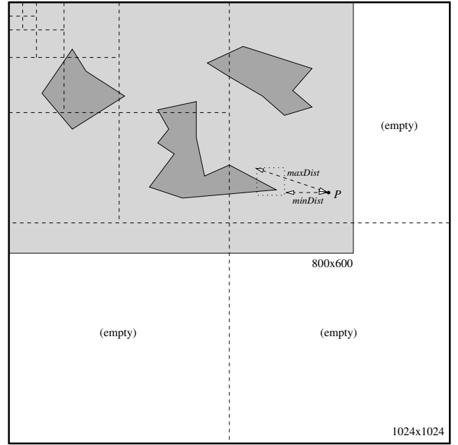
Figure 2: Quadtree representation of a semantic object buffer. The dotted rectangle shows an example spatial query for a node where the minimum and maximum possible distances from the pointer P are computed.
