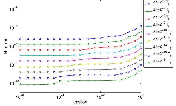
(b) Error with respect to \epsilon
