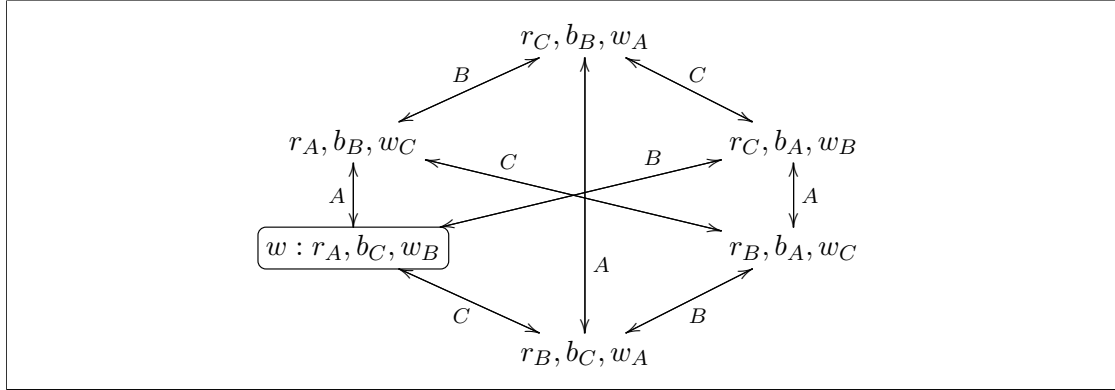
Figure 1: Cards Example
