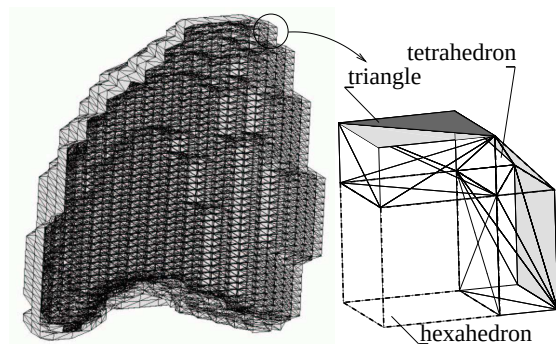
Figure 8. tetrahedral, triangle and hexahedral mesh (a.), detail (b.)
