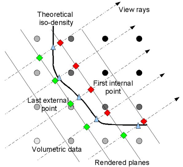
Figure 7: Isosurface estimation
