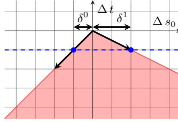
Figure 4: Opposite dependence cone
