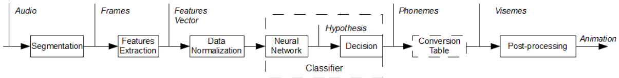
Figure 1: Illustration of the speech driven lip animation system.
