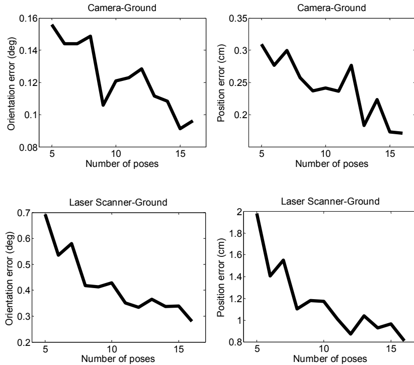
Fig.2. The influence of the number of chessboard poses
