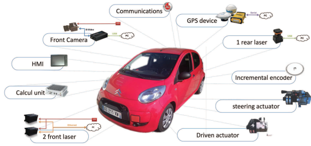
Fig. 1. Vehicle equipment
