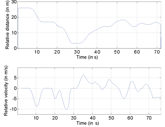
Fig. 9. Front obstacle relative distance and velocity
