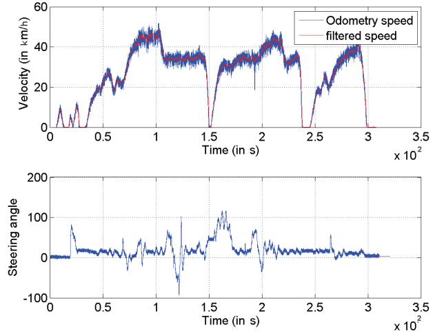
Fig. 8. Vehicle velocity
