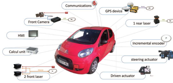
Fig. 1. Vehicle equipment
