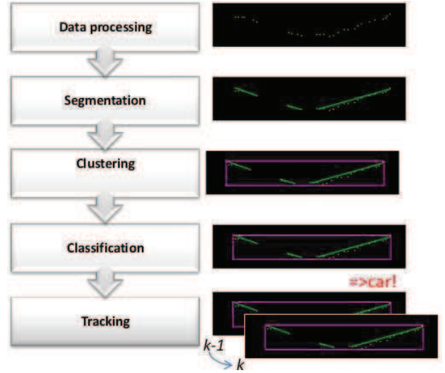
Fig. 4. Obstacle detection and tracking: general scheme
