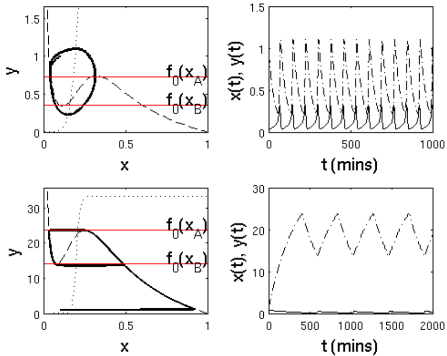
Figure 5: Periodic orbit and trajectories for system, with parameters as in Table 2 (top row), or with the parameters listed above (bottom row), which enhance the difference between timescales.
