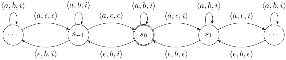
Figure 7: CCSL Inf (infinite state LTS): i \triangleq \mathbf{Inf}(a, b) .
