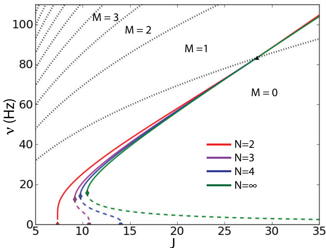
Figure 2. Frequencies of the splay states as a function of the synaptic strength J and for pulse duration T_s N = 12 ms with \tau = 20 ms. Red line: N = 2 , magenta line: N = 3 , blue line: N = 4 , green line: N = \infty . Black dotted lines separate regions with different numbers M of overlapping PSPs. Solid lines refer to the upper stable branches of the splay state. Dashed lines refers to the lower unstable branches of the splay state. For N = 2 the lower branch does not exist.
