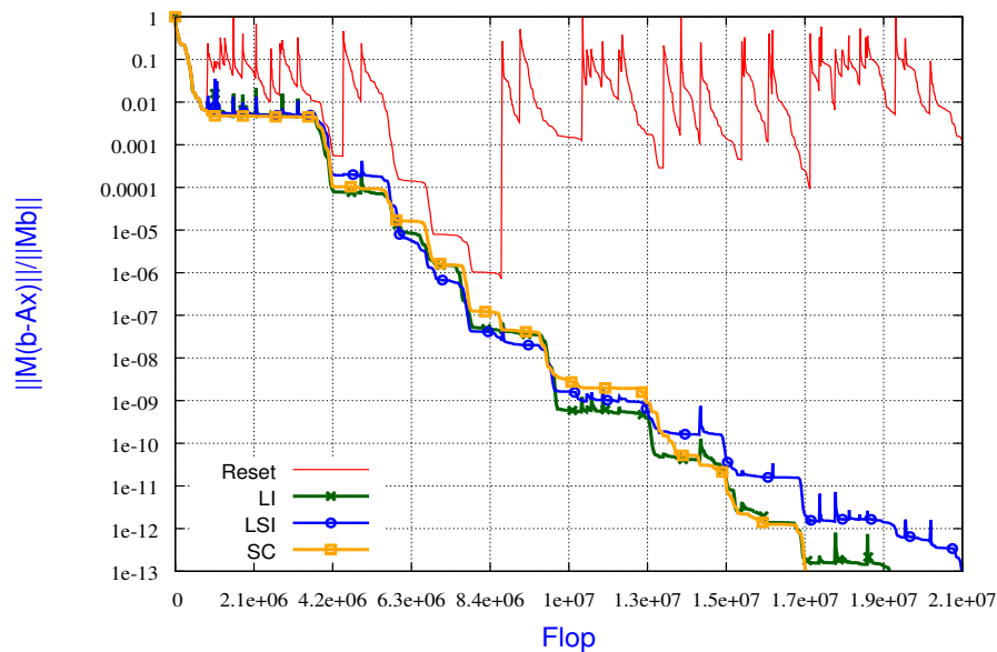
Figure 13: Left preconditioned GMRES on Averous/epb0 using 16 processors with 44 single faults
