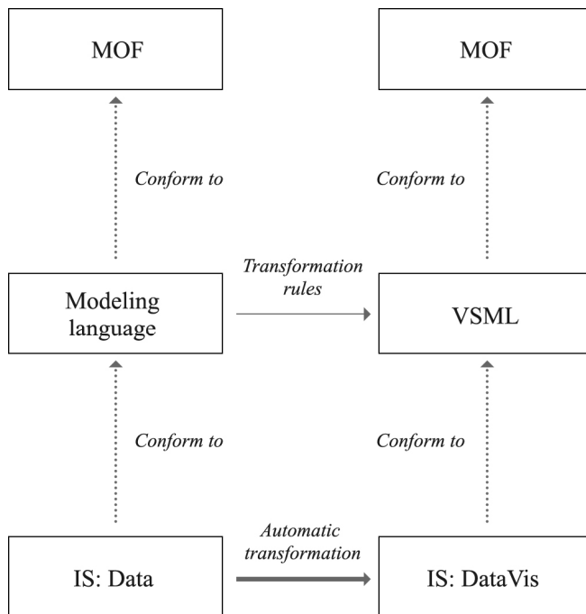
Figure 4. VSML transformation
