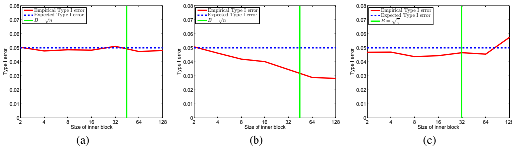
Figure 2: Empirical number of Type I errors on the distributions shown in Figure 3 for \alpha = 5\% : (a) MMD, single kernel, \sigma = 1 , (b) MMD, single kernel, \sigma set to the median pairwise distance, and (c) MMD, non-negative linear combination of multiple kernels. The experiment was repeated 30000 times. Error bars are not visible at this scale.
