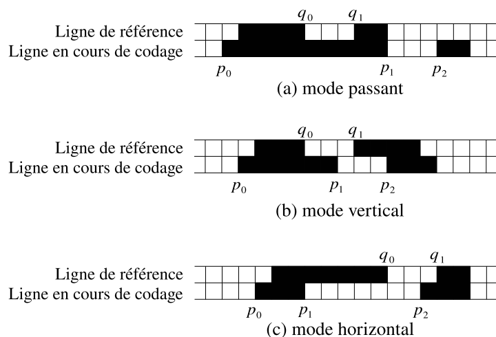
Figure 3.22. Codage RLC-2D
