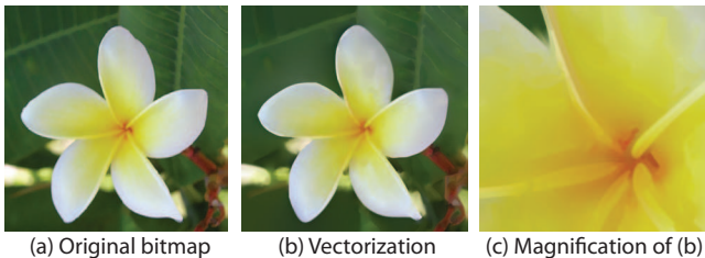
Figure 8: Automatic vectorization.
