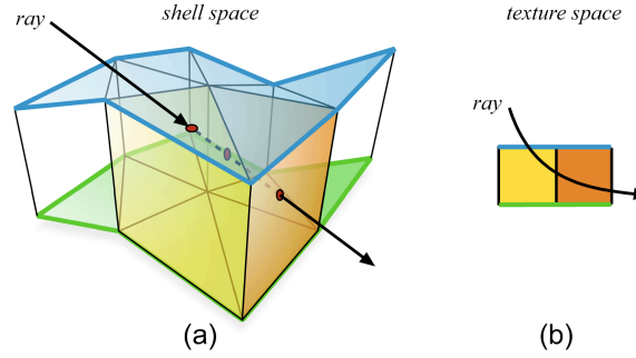
Fig. 7. Linear ray in shell space is a curved ray on texture space [Porumbescu et al., 2005].
