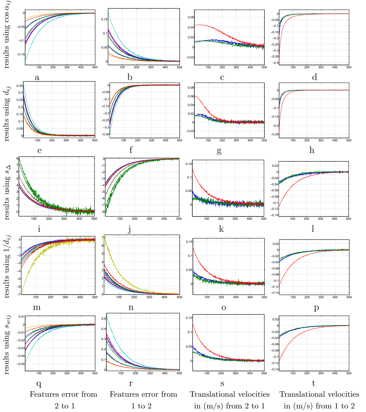
Figure 6: Simulation results when only translational motions are controlled
