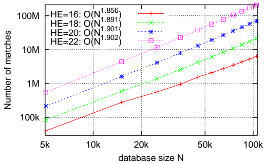
Figure 1: Number of collected matches sketches for varying image set size and of threshold h_t ( M = 768 ). The complexity is empirically estimated for all h_t .
