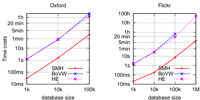
Figure 3: Timings for linking an image collection.
