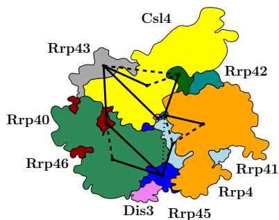
C MILP
